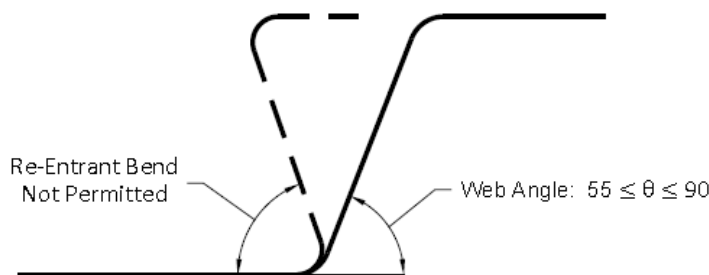
Figure C-F3.2-1 – Limit on Deck Web Angle for Prequalified Method
