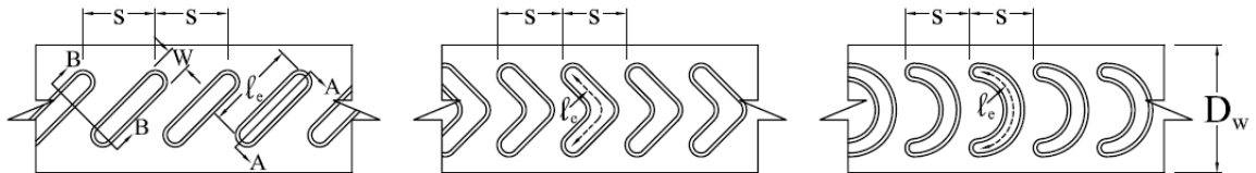
Figure F3.2-1 – Type 1 Embossments with length measured along centerline
