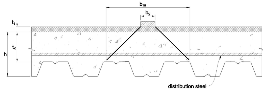
Figure C-F6-1 – Lateral Distribution
