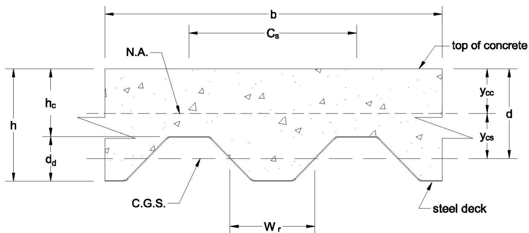
Figure C-F2.3-1 – Composite Section
