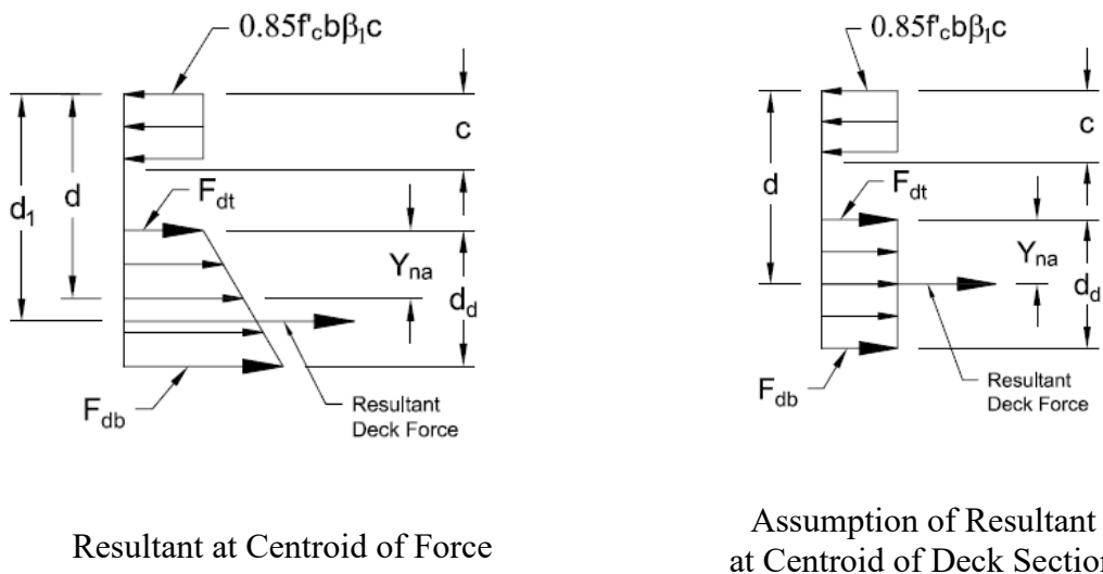
Figure C-F3.1-2 – Centroid of Force in Deck Section
