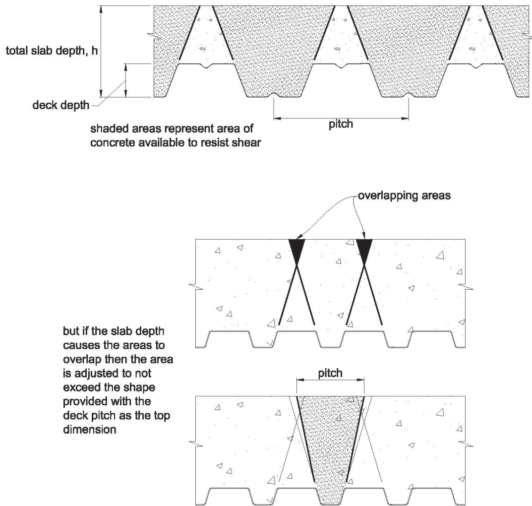
Figure F4-1 – One-Way Shear Parameters - Web Angle < 90 Degrees
