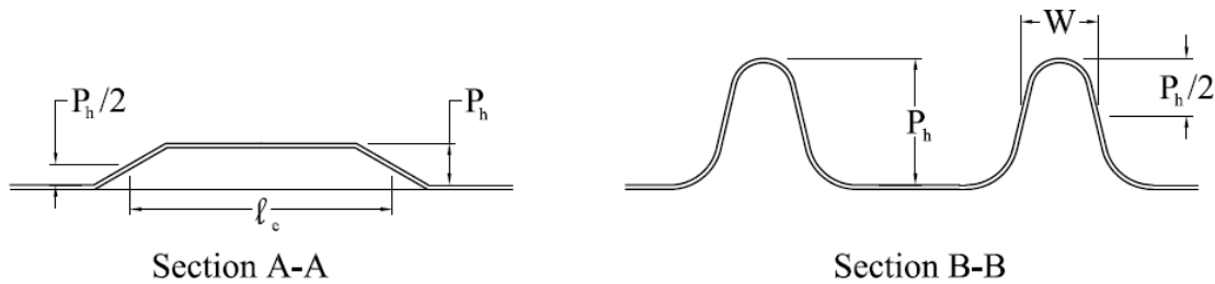
Figure F3.2-4 – Embossment Section Details
