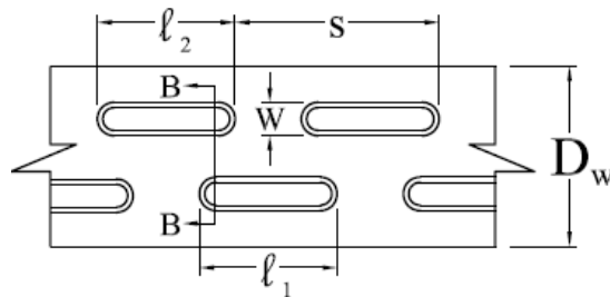
Figure F3.2-2 – Type 2 Embossments
