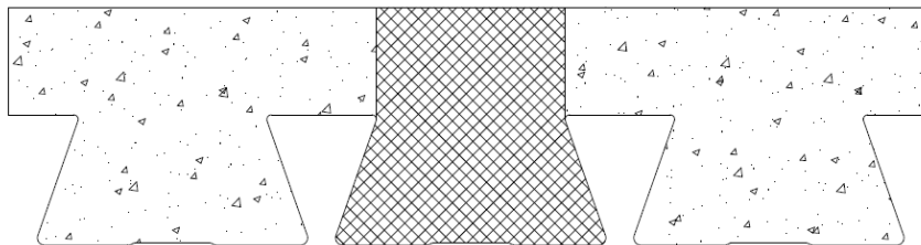
Figure F4-2 – One-Way Shear Parameters - Web Angle \geq 90 Degrees
