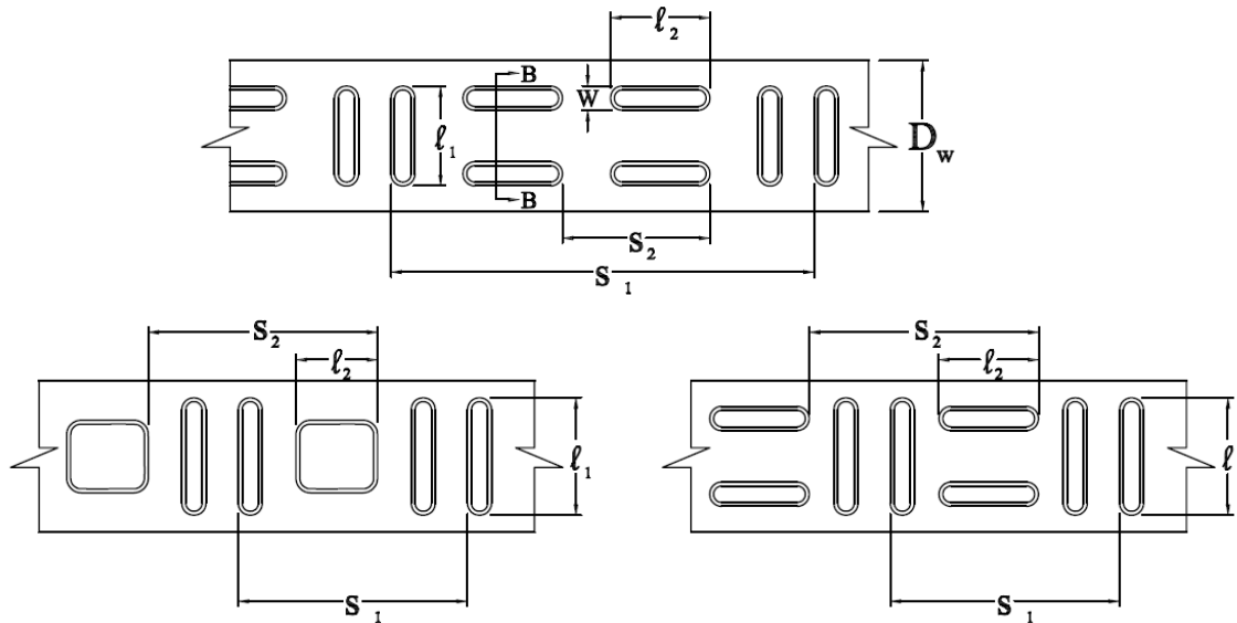
Figure F3.2-3 – Type 3 Embossments
